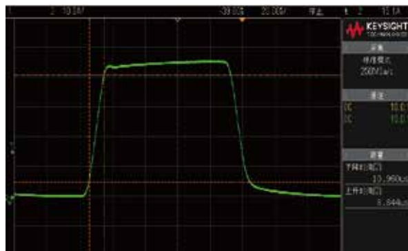
IT8723P+从1A到45A动态波形，设定电流斜率4.5A/ \mu s
